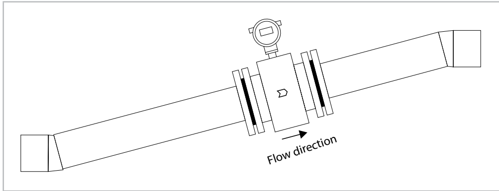
Fig 7: Horizontal Installation
