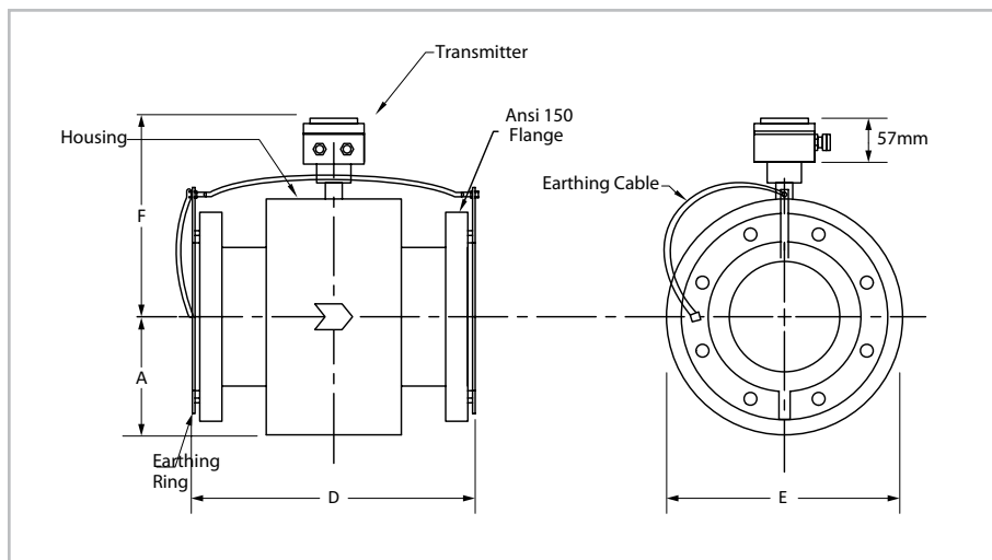
Fig 5: Remote Type
